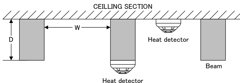
Figure 9: Heat detector spacing — beam construction (side view)
