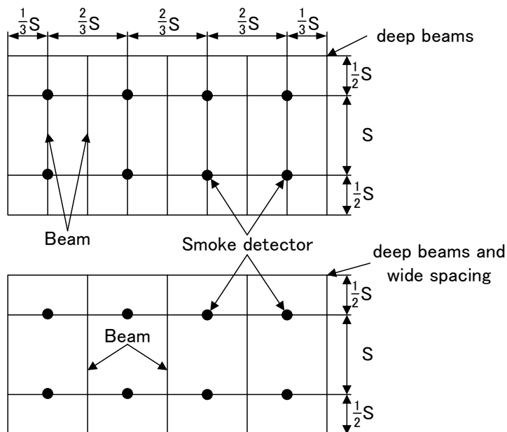
Figure 17: Smoke detector spacing — beam construction (plan view)
